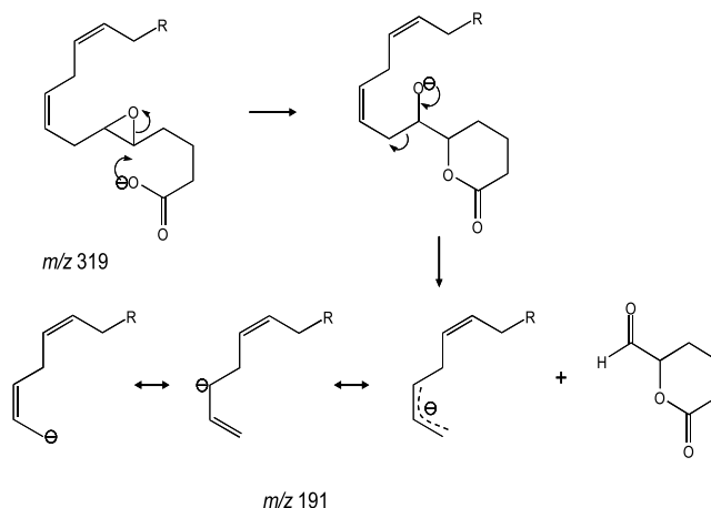
Figure 3. Fragmentation pattern explaining origins of ions m/z 191 from the collisionally activated dissociation of the molecular 5,6-EET carboxylate anion at m/z 319. R = C 10 H 17 .
