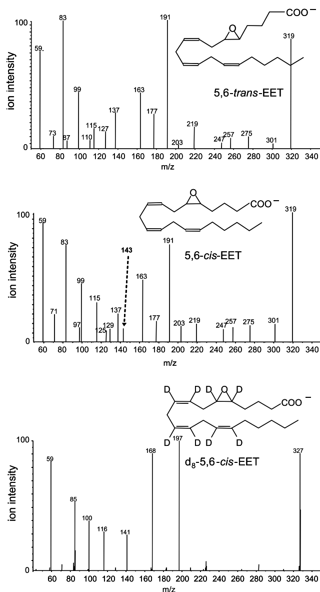
Figure 1. Comparison of tandem mass spectra obtained by collisional activation at -30 V of the carboxylic anion at m/z 319 generated from 5,6- trans -EET (top), 5,6- cis -EET (middle) and of ion m/z 327 from octadeuterium-labeled 5,6- cis -EET (bottom), which were prepared by iodolactonization of 5,6- trans -AA, AA, and d 8 -AA, respectively. The spectra were averaged and background noise was subtracted.
