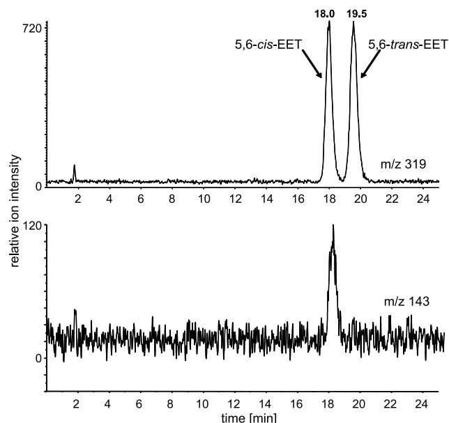
Figure 5. LC–MS analysis showing separation of cis and trans isomers of 5,6-EET with selected acquisition of ions at m/z 319 and 143. The latter appears only in the cis isomer. Lipids were analyzed on a Phenomenex Luna C18 column (150 × 2 mm) and eluted with a solution composed of water–acetonitrile–acetic acid (37.5:62.5:0.01 v/v/v) at a rate of 300 μL/min. Lipids were ionized and detected by the API 2000 mass spectrometer operating in a turbo-ion spray negative mode.
