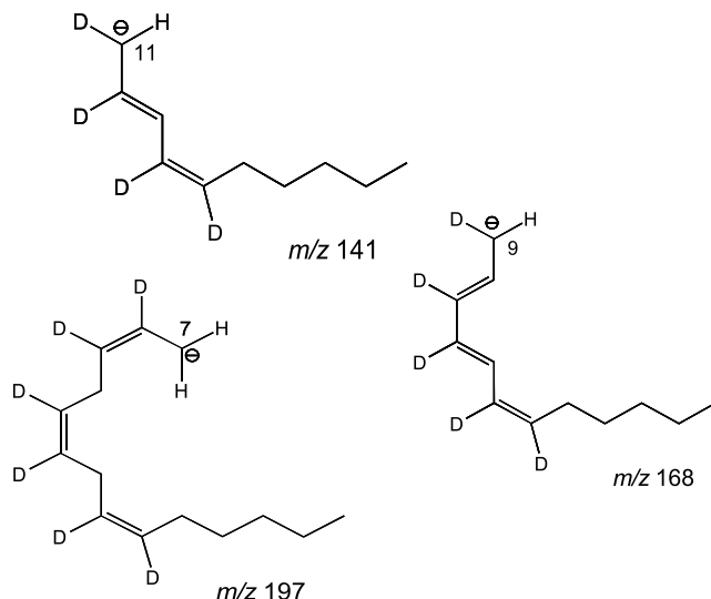
Figure 4. Structures of three major fragment ions observed in the spectrum of d 8 -5,6- cis -EET (Fig. 1). The structures are hypothetical and are likely to involve other resonance structures. Corresponding ions in the spectrum of 5,6- cis -EET are found at m/z 137, 163, and 191 suggesting that the ions had four, five, and six deuterium, respectively.
