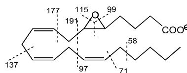
Figure 2. Fragmentation pattern of 5,6- trans -EET carboxylate anion resulting from collisional activation of ion m/z 319 generating a spectrum shown in Figure 1.
